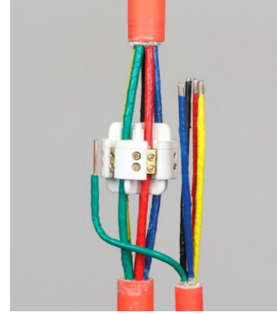
5 Install the branch cables
