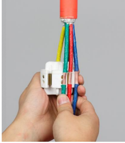
4 Install the branch cable body
